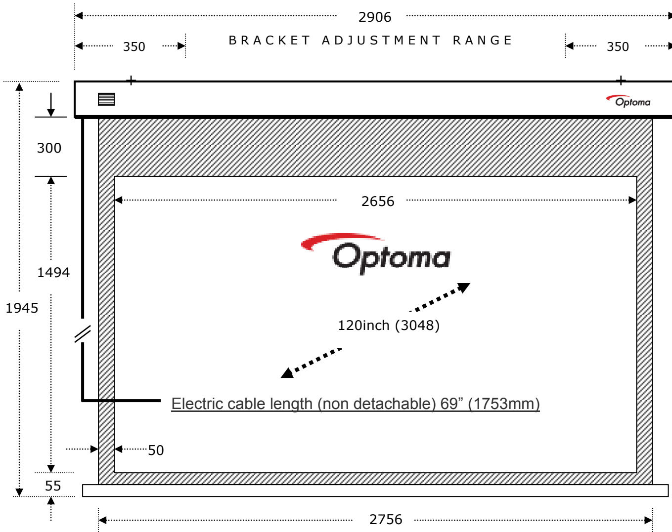
OPTOMA DE-9120EGA ELECTRIC Measurements in Milimetres
